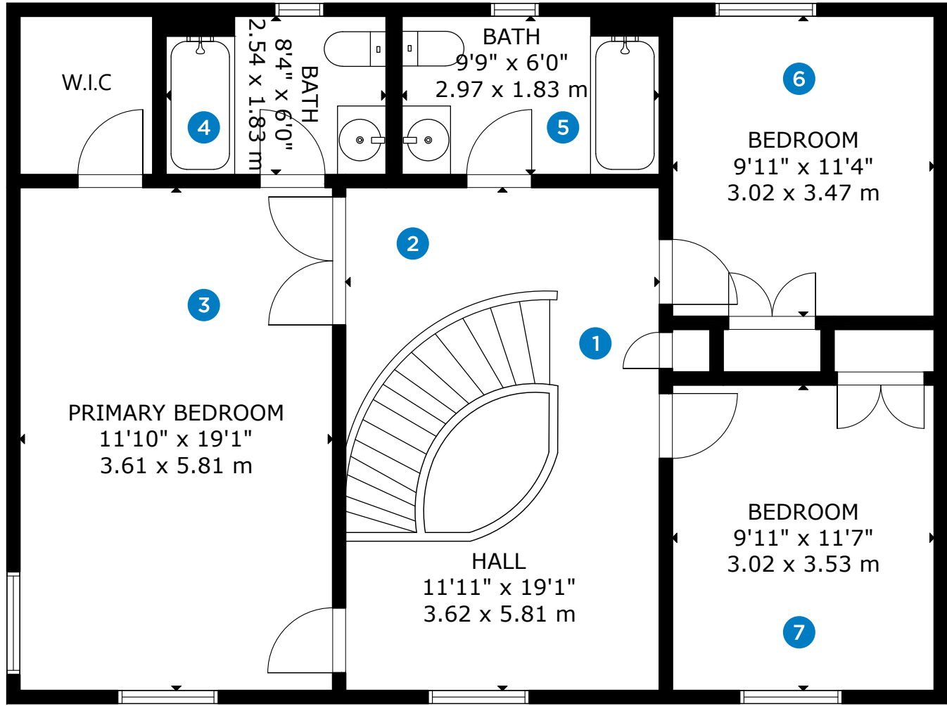
UPPER LEVEL: 945 SQUARE FEET
